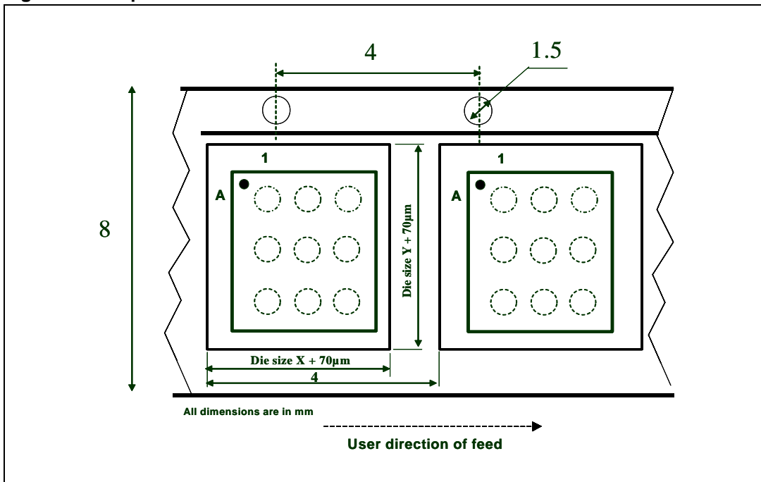
Figure 102. Tape & reel dimensions
