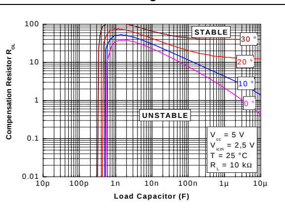
Figure 29. Phase margin abacus : serial resistor to be added in a voltage follower configuration at 25°C
