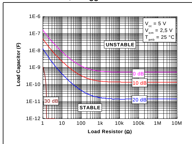
Figure 19. Gain margin according the output load, at V_{CC}=5V and T=25^{\circ}C
