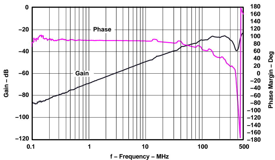
Figure 4. Frequency Response vs Crosstalk
