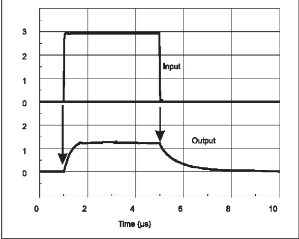
Pulse Response for I_k = 100\mu\text{A}
