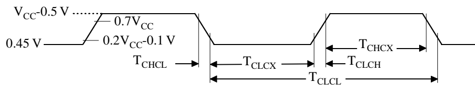
Figure 30. External Clock Drive Waveforms
