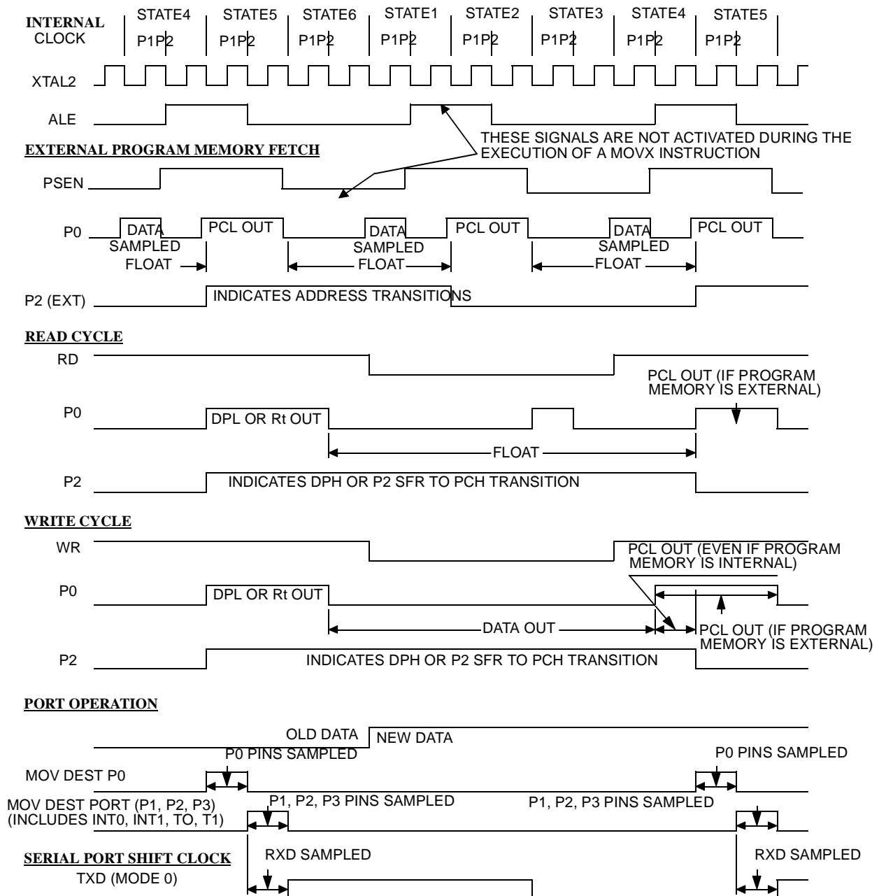
Figure 33. Clock Waveforms
