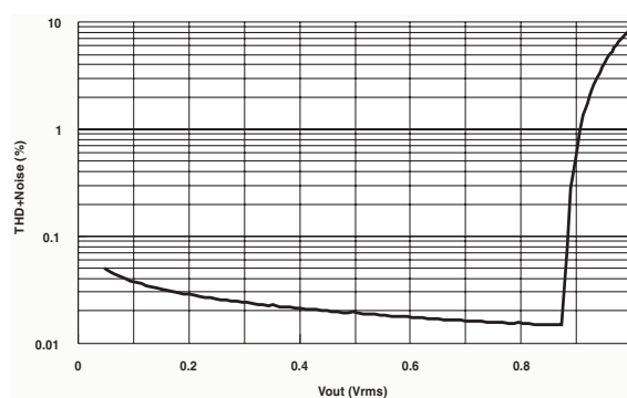
Figure 8. THD + noise vs. output voltage
