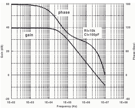
Figure 2. Voltage gain and phase vs. frequency
