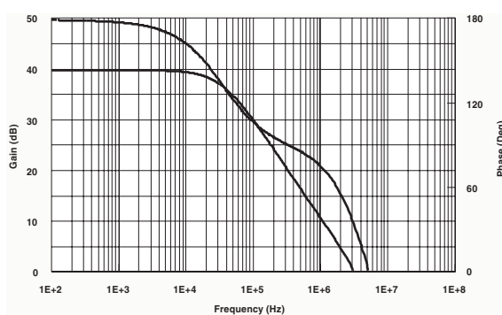
Figure 12. Open loop gain and phase vs. frequency
