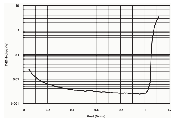
Figure 10. THD + noise vs. output voltage
