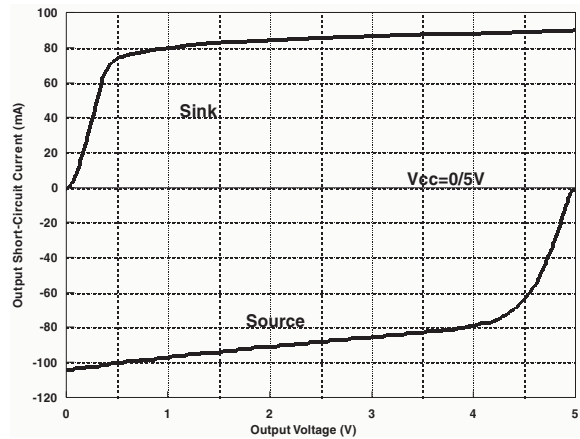
Figure 1. Output short circuit vs. output voltage
