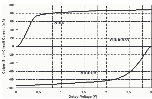
Figure 3. Output short circuit vs. output voltage
