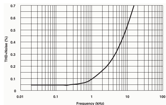
Figure 9. THD + noise vs. frequency
