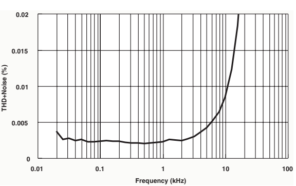
Figure 6. THD + noise vs. frequency
