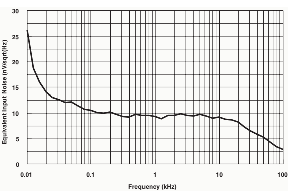
Figure 4. Equivalent input noise voltage vs. frequency
