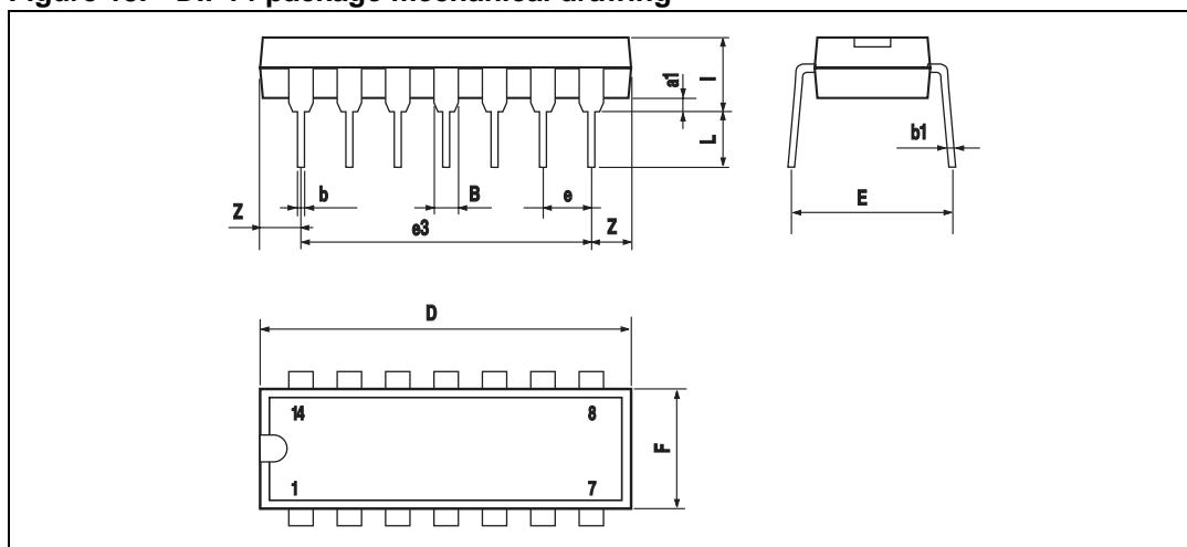
Figure 13. DIP14 package mechanical drawing
