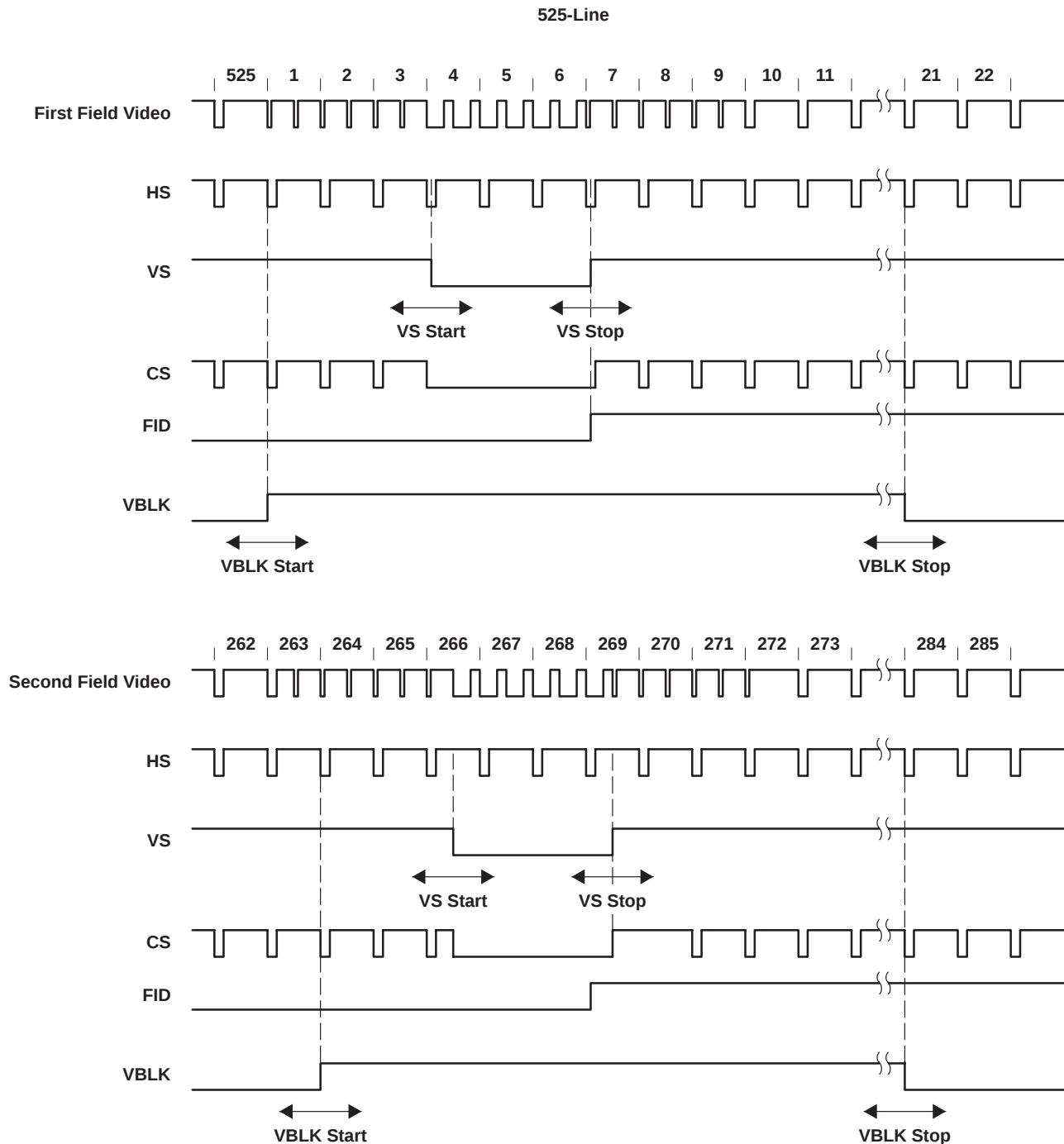
Figure 2–14. Vertical Synchronization Signals for 525-Line System
