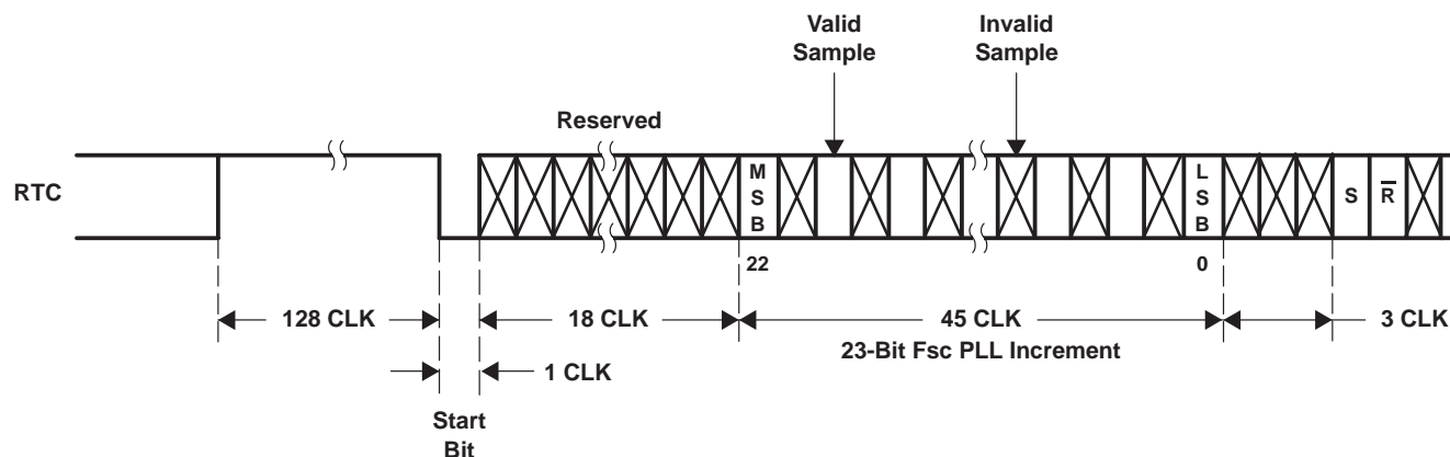
Figure 2–11. RTC Timing
