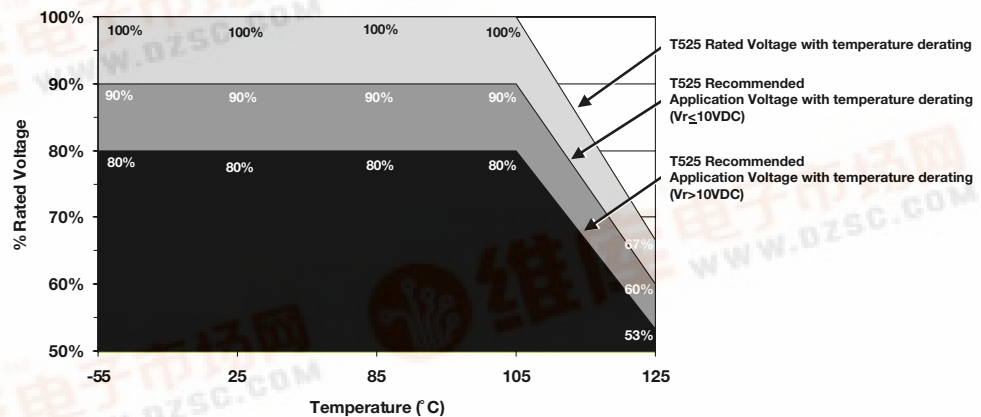
T525 Temperature/Application Recommended Voltage Derating
