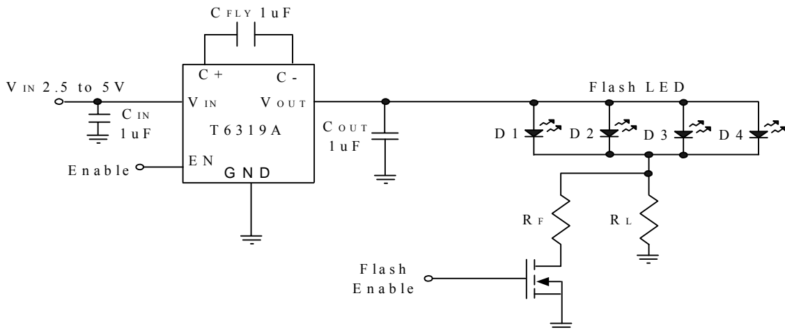
Flash LED Driver with Gated Flash Application
