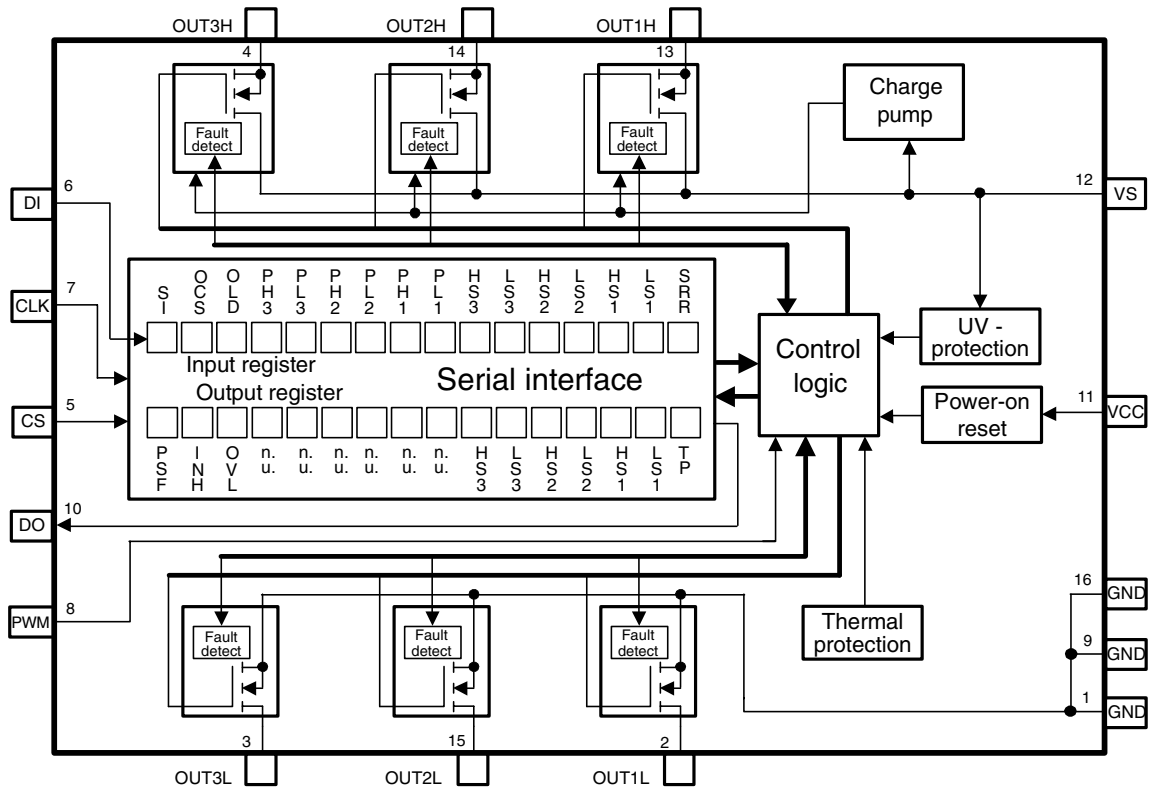
Figure 1. Block Diagram
