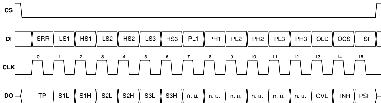
Figure 3. Data Transfer
