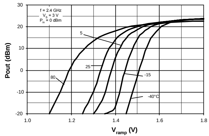
Figure 7. P_{\text{out}} versus V_{\text{ramp}} and Temperature
