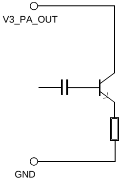
Figure 13. Input/Output Circuit V3_PA_OUT
