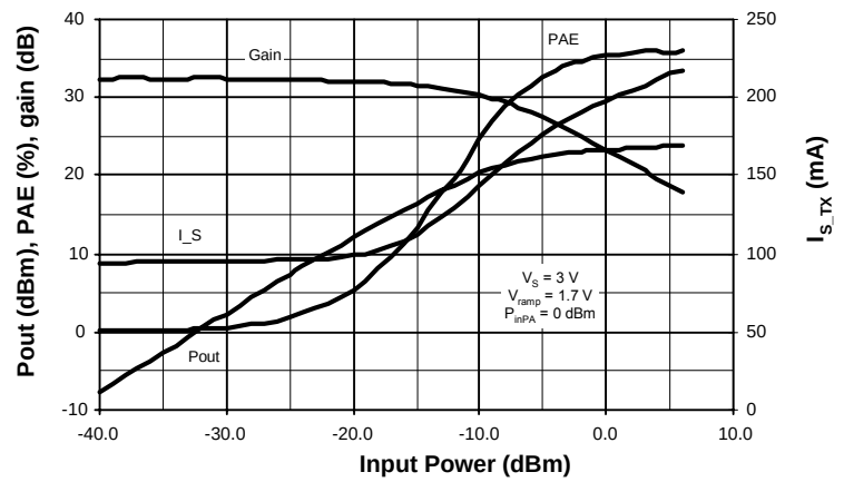
Figure 6. Output Power and PAE versus Input Power
