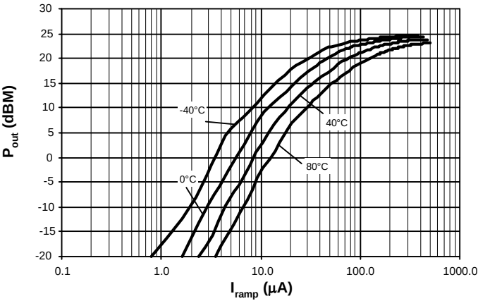
Figure 8. Output Power versus I_{\text{Ramp}} Current
