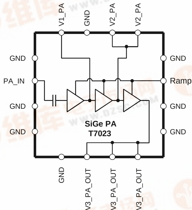
Figure 1. Block Diagram
