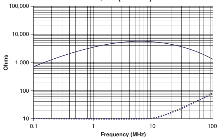
Impedance in Common Mode and Differential Mode T8112 (2 x 1mH)
