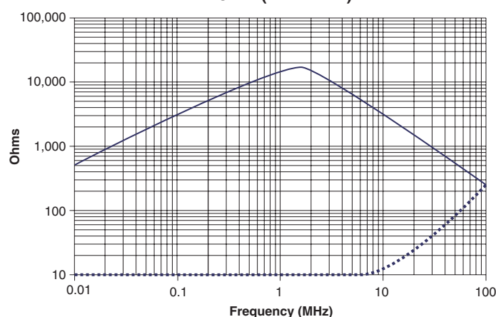
Impedance in Common Mode and Differential Mode T8114 (2 x 4.7mH)
