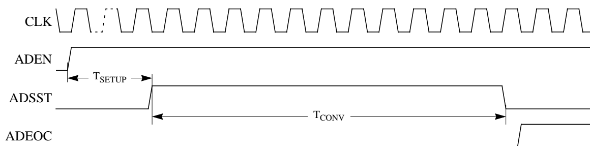
Figure 78. Timing Diagram
