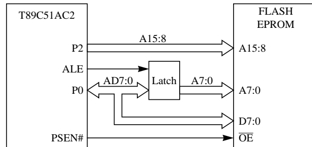
Figure 9. External Code Memory Interface Structure
