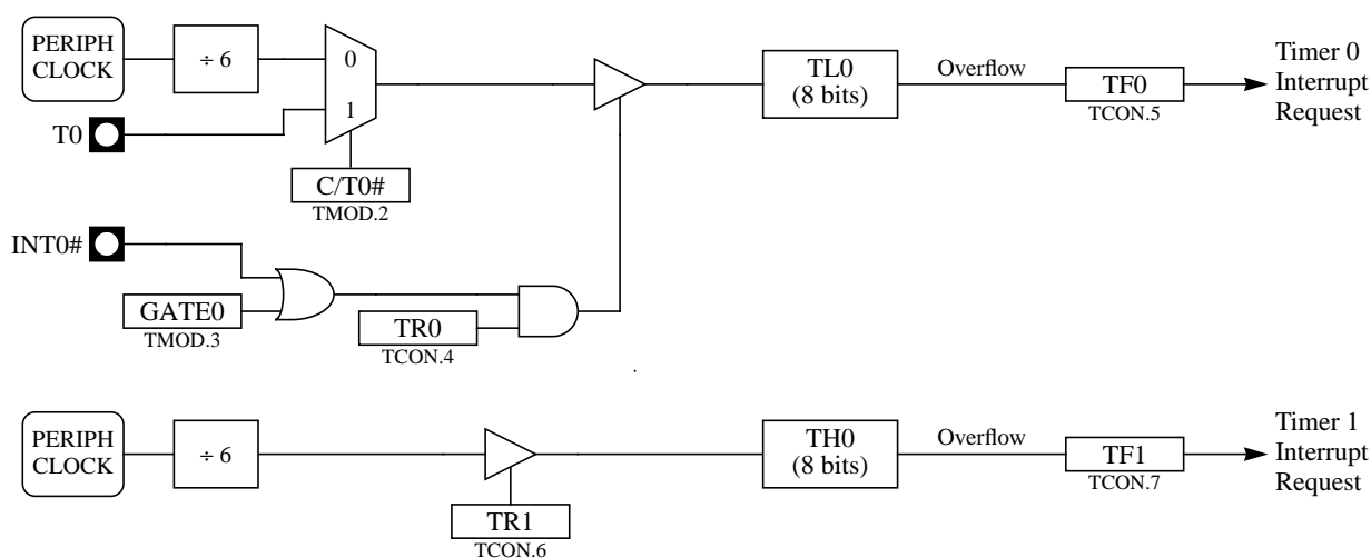
Figure 45. Timer/Counter 0 in Mode 3: Two 8-bit Counters
