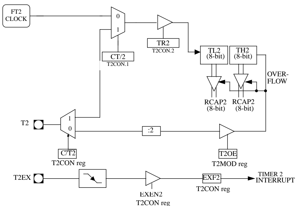
Figure 54. Clock-Out Mode
