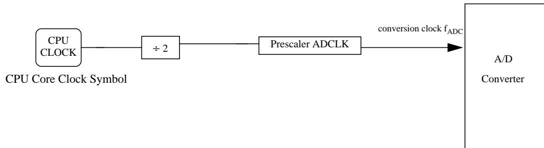
Figure 79. A/D Converter clock
