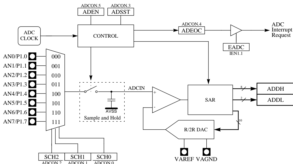
Figure 77. ADC Description
