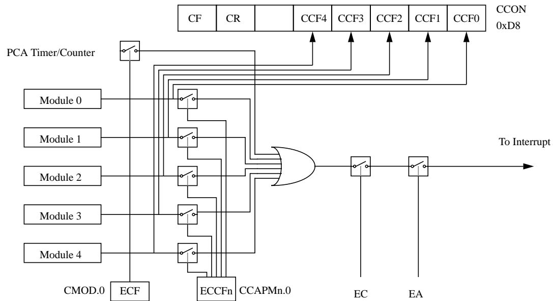
Figure 65. PCA Timer Interrupts
