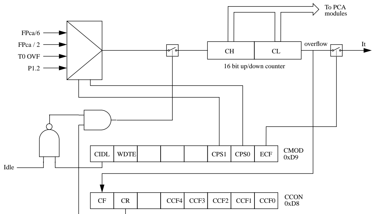
Figure 64. PCA Timer/Counter
