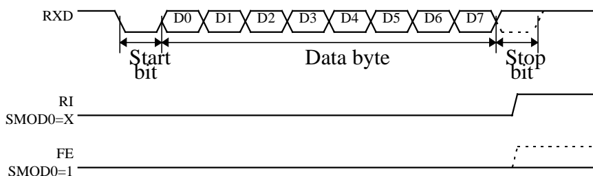
Figure 35. UART Timing in Mode 1
