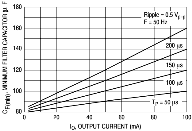
Figure 13. Minimum Filter Capacitor versus Output Current
