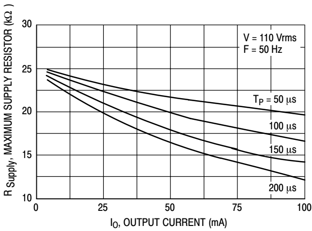
Figure 11. Maximum Supply Resistor versus Output Current
