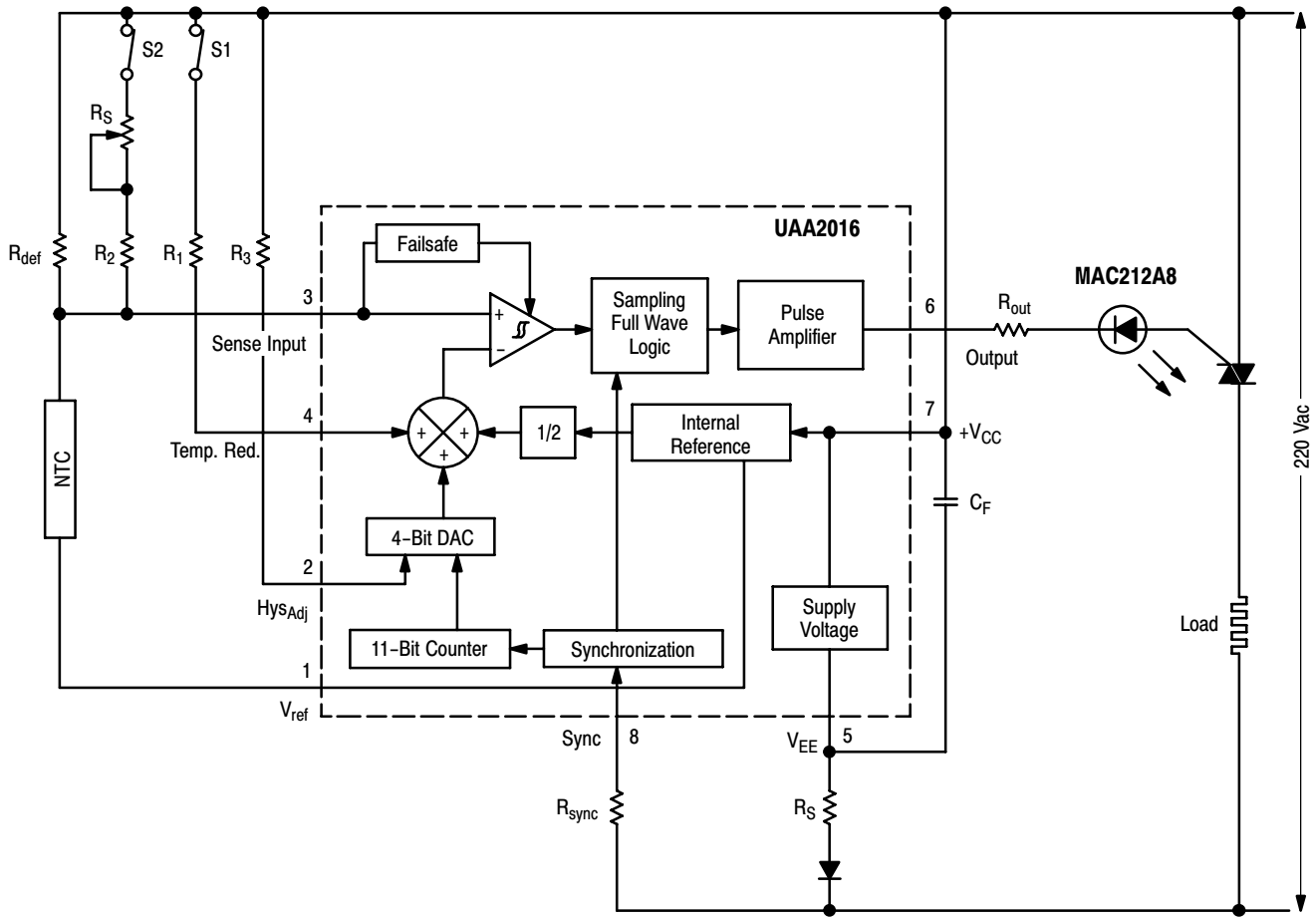
Figure 1. Application Schematic
