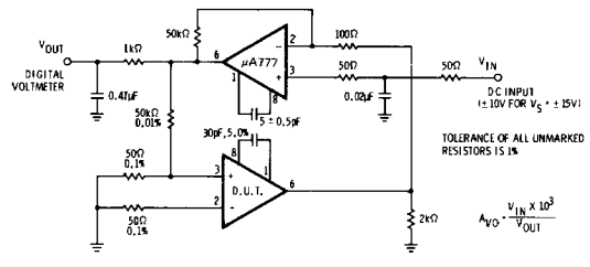
GAIN TEST CIRCUIT
