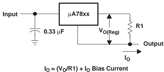
Figure 4. Current Regulator
