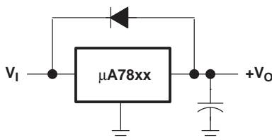
Figure 7. Reverse-Bias-Protection Circuit
