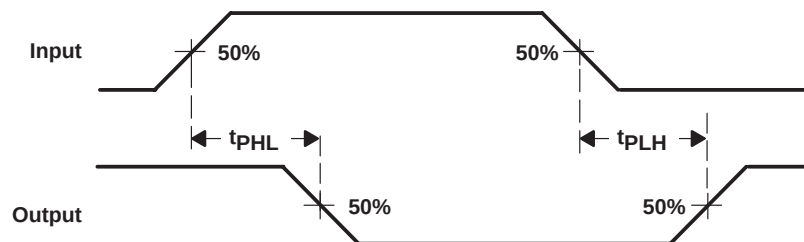
Figure 9. Propagation Delay-Time Waveforms
