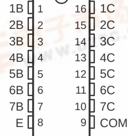
D, N, OR NS PACKAGE (TOP VIEW)
