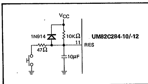
Figure 2. Typical RC \overline{RES} Timing Circuit
