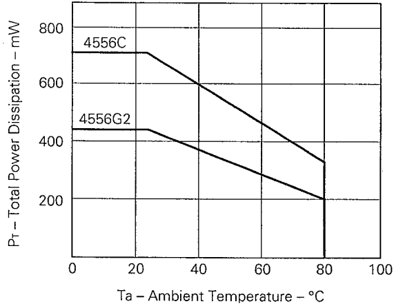
POWER DISSIPATION
