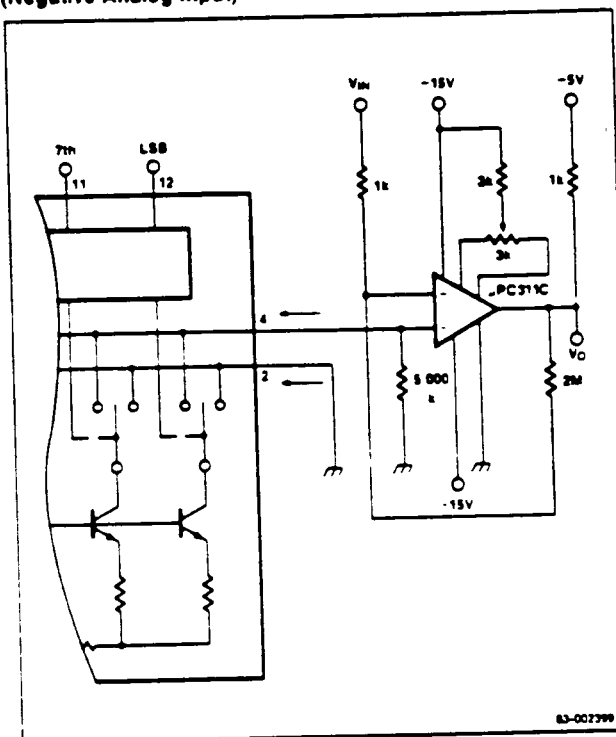
Comparator Connection Method for A/D Conversion (Negative Analog Input)
