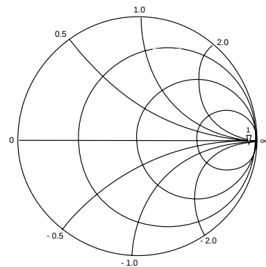
Limiter Amp Input Impedance (Pin 14) 1. 10.7 MHz: 1.3k + j246.8
