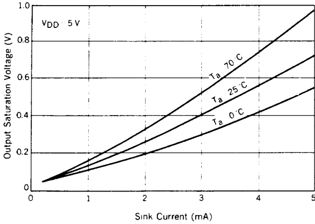
OUTPUT SINK CURRENT vs. SATURATION VOLTAGE CHARACTERISTICS
