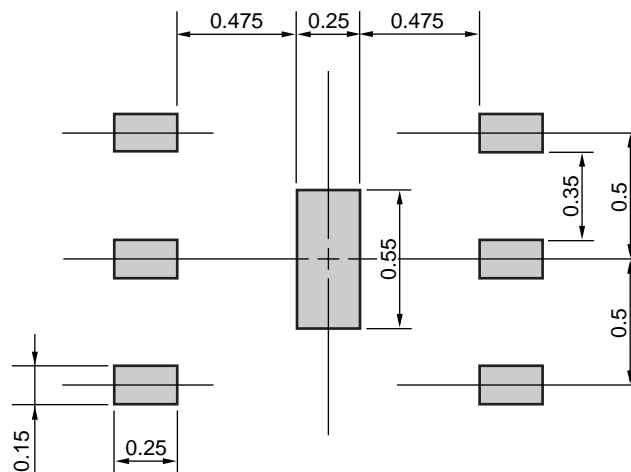
SOLDER PAD
