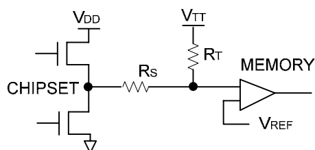
Figure 1. SSTL-Termination Scheme
