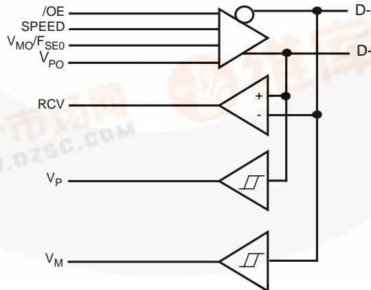
Figure 1. Logic Diagram
