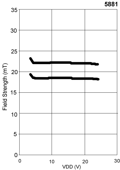
11.1 Typical Magnetic Switch Points vs V_{DD}
