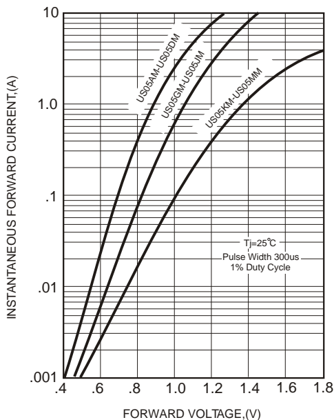
FIG.4-Typical Forward Characteristics
