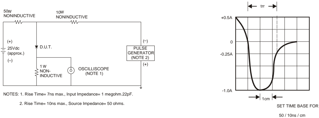
FIG.1- Test Circuit Diagram and Reverse Recovery Time Characteristics
