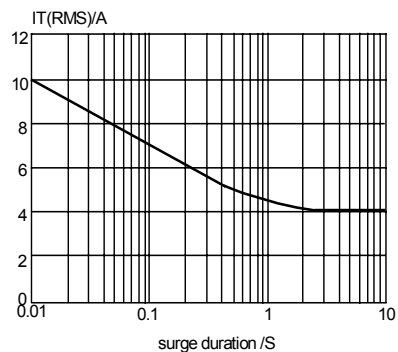
Fig.5. Maximum permissible repetitive rms on-state current I_T(RMS) , vs surge duration, for sinusoidal currents, f=50\text{Hz} ; T_{mb} \leq 107^\circ\text{C}
