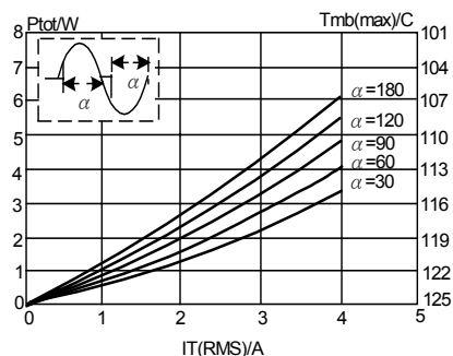
Fig.1. Maximum on-state dissipation, P_{tot} vs rms on-state current, I_T(RMS) where \alpha = conduction angle.
