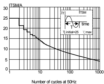
Fig3. Maximum Permissible non-repetitive peak on-state current I_{TSM} , vs number of cycles, for sinusoidal currents, f=50\text{Hz} .
