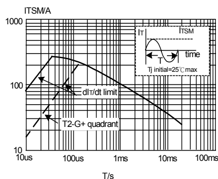
Fig.2. Maximum Permissible non-repetitive peak on-state Current I_{TSM} vs pulse width t_p , for sinusoidal currents, t_p \leq 20\text{ms}
