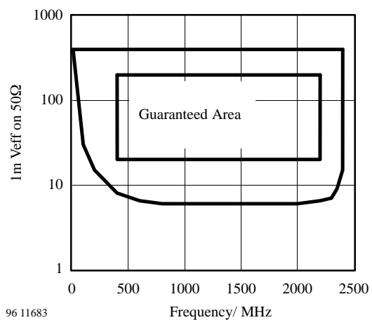
Figure 8. Input sensitivity of PLL1
