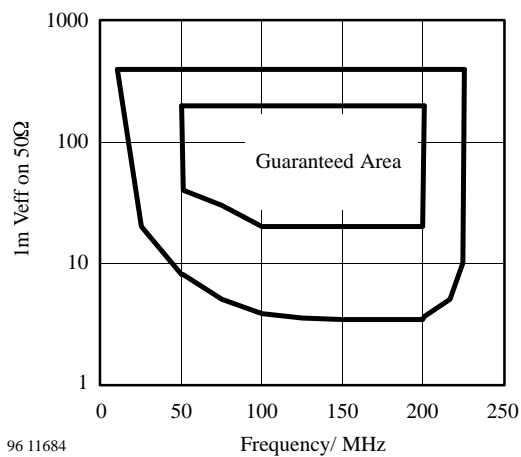
Figure 9. Input sensitivity of PLL2
