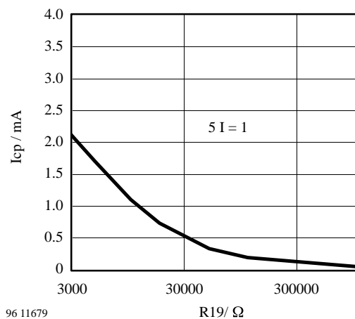
Figure 7. Charge pump characteristics
