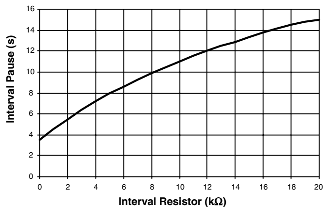
Figure 8-3. Interval Pause = f(R_{\text{INT}}) ; C_t = 22 \mu\text{F}
