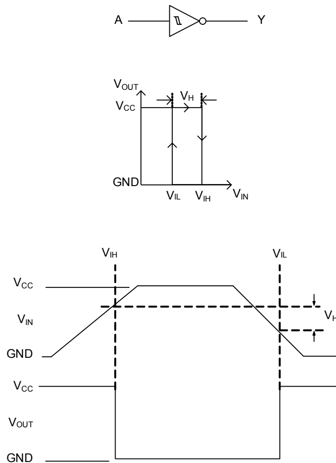
Figure 1. Hysteresis Definition, Characteristic, And Test Setup
