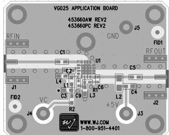
Circuit Board Material: .014" FR-4, 4 layers, .062" total thickness
