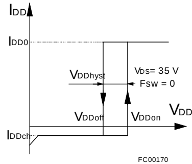
Figure 8. Shutdown Action
