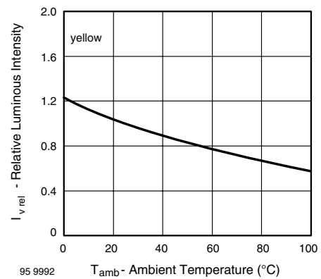
Figure 15. Relative Luminous Intensity vs. Ambient Temperature
