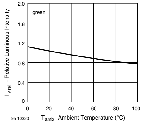
Figure 20. Relative Luminous Intensity vs. Ambient Temperature
