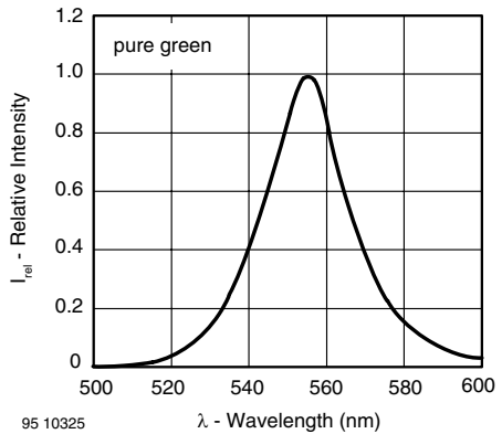
Figure 28. Relative Intensity vs. Wavelength
