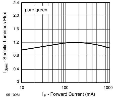
Figure 26. Specific Luminous Intensity vs. Forward Current
