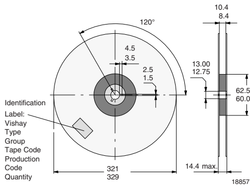
Figure 31. Reel Dimensions - GS18
