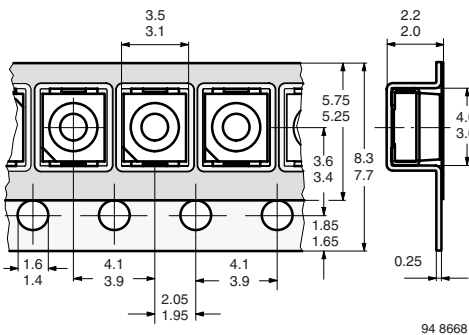
Figure 6. Tape Dimensions in mm for PLCC-2
