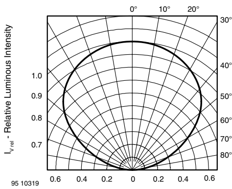
Figure 8. Rel. Luminous Intensity vs. Angular Displacement
