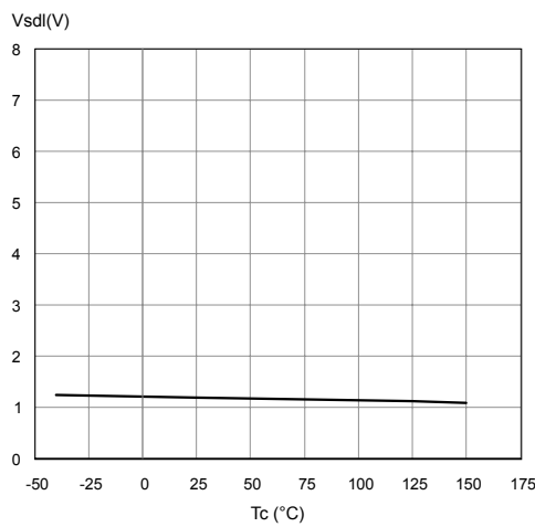
Figure 27. Low Level STAT_DIS Voltage
