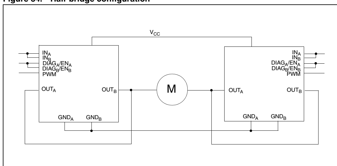
Figure 34. Half-bridge configuration
