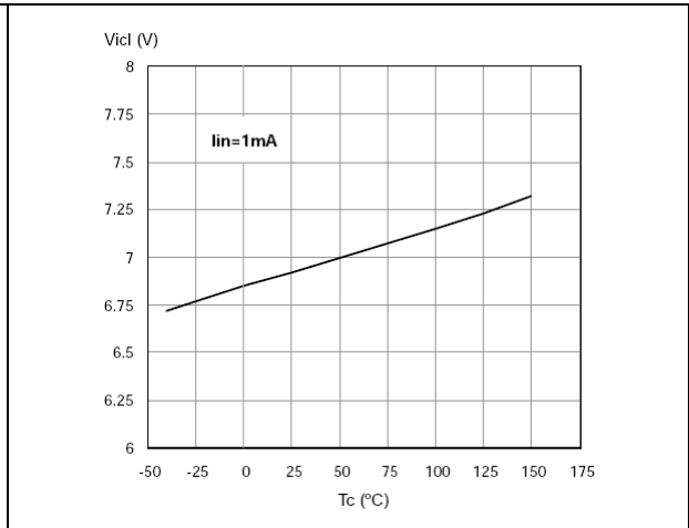
Figure 10. Input clamp voltage
