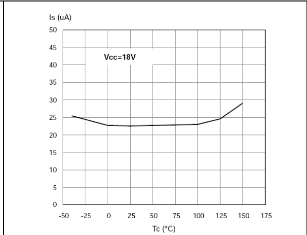
Figure 8. Off state supply current
