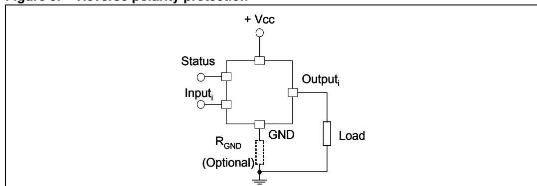
Figure 9. Reverse polarity protection
