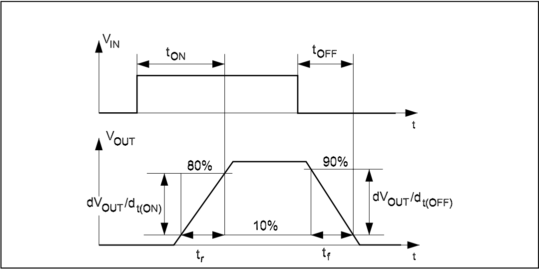
Figure 4. Switching characteristics
