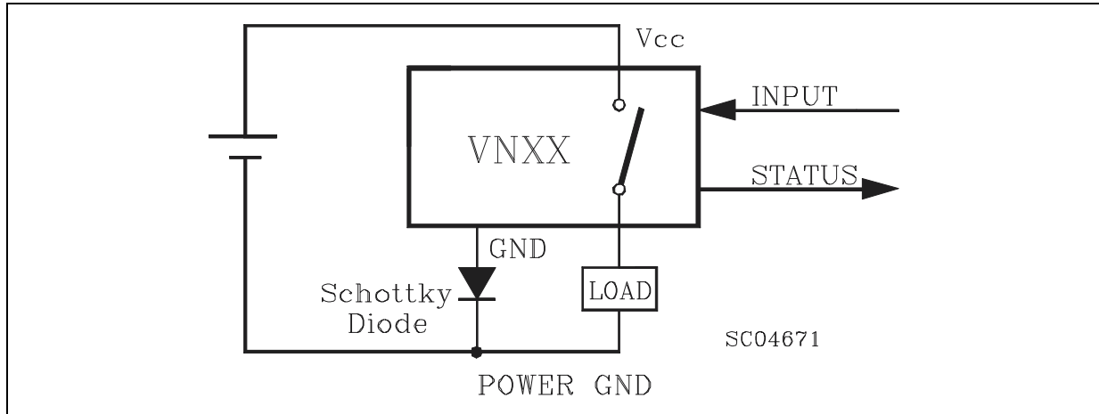
Figure 10. Typical Application Circuit With A Schottky Diode For Reverse Supply Protection
