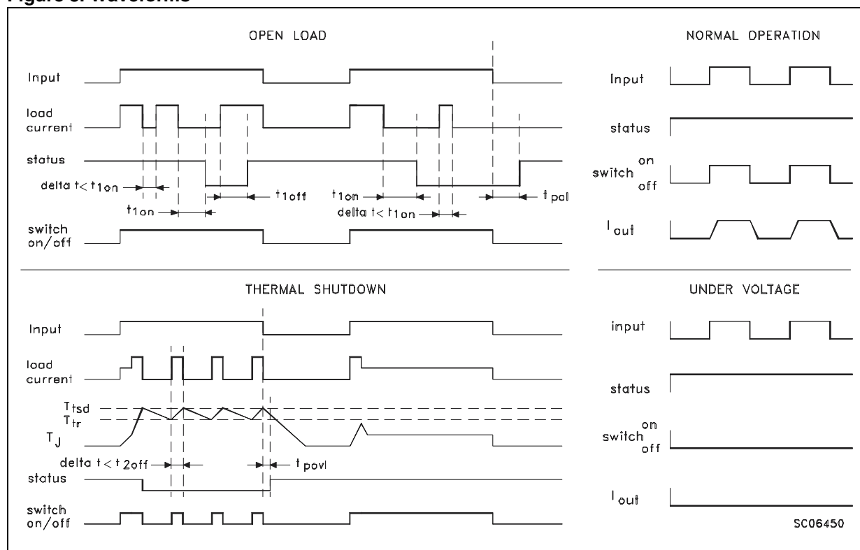
Figure 8. Waveforms
