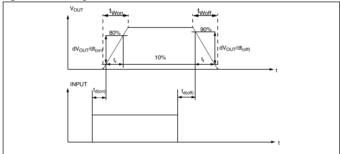
Figure 8. Switching characteristics
