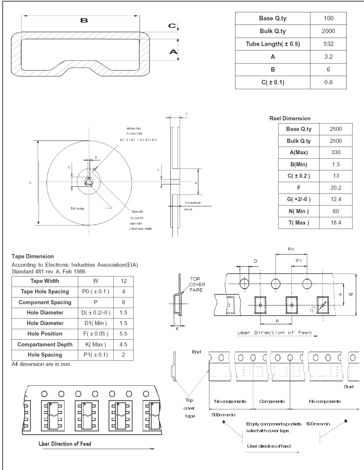
Figure 11. SO-8 tape and reel information
