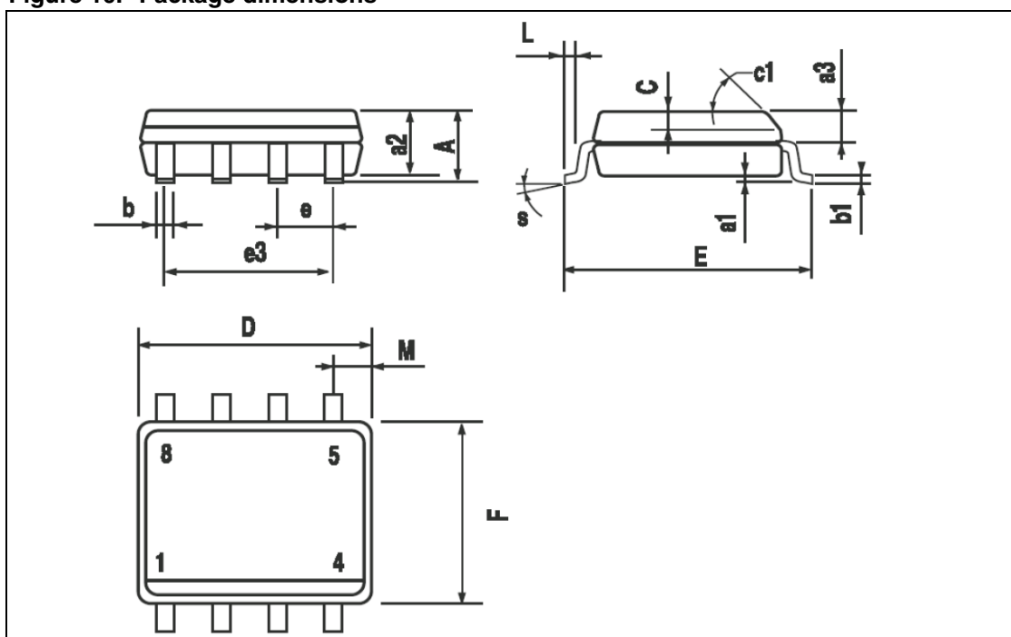
Figure 10. Package dimensions
