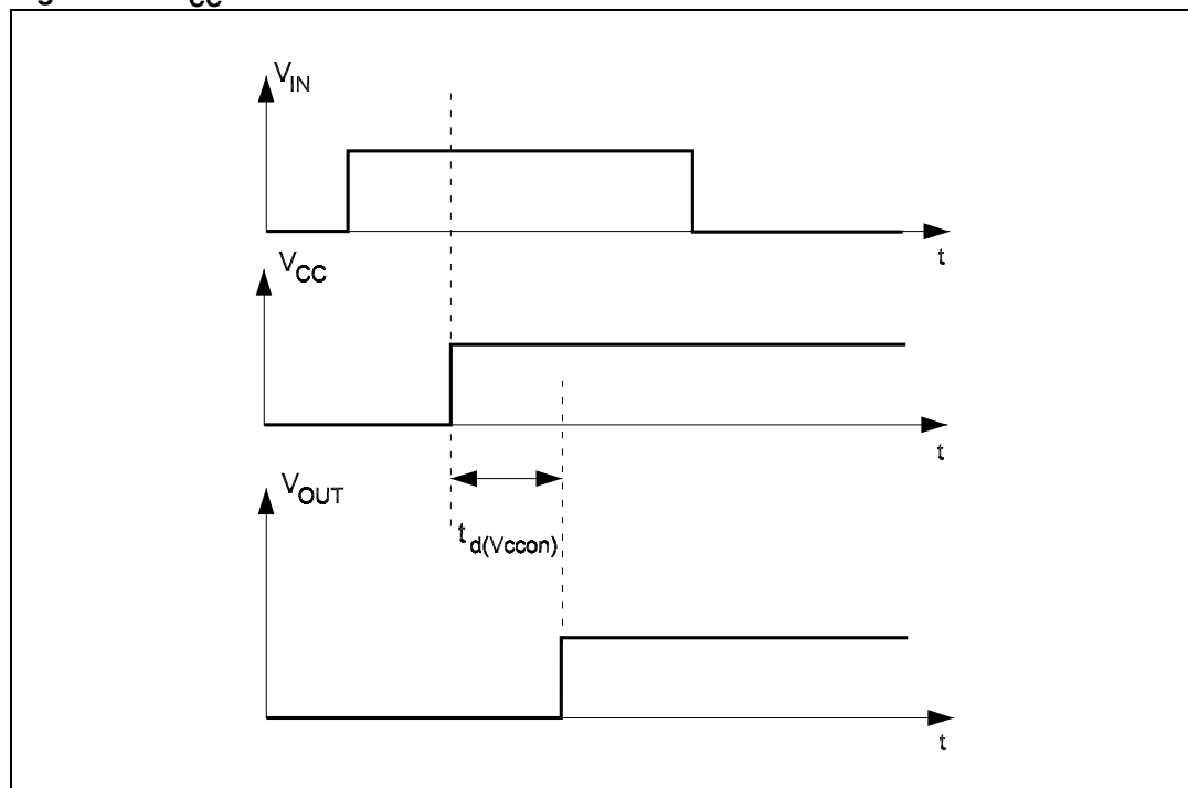
Figure 6. V_{CC} turn-ON
