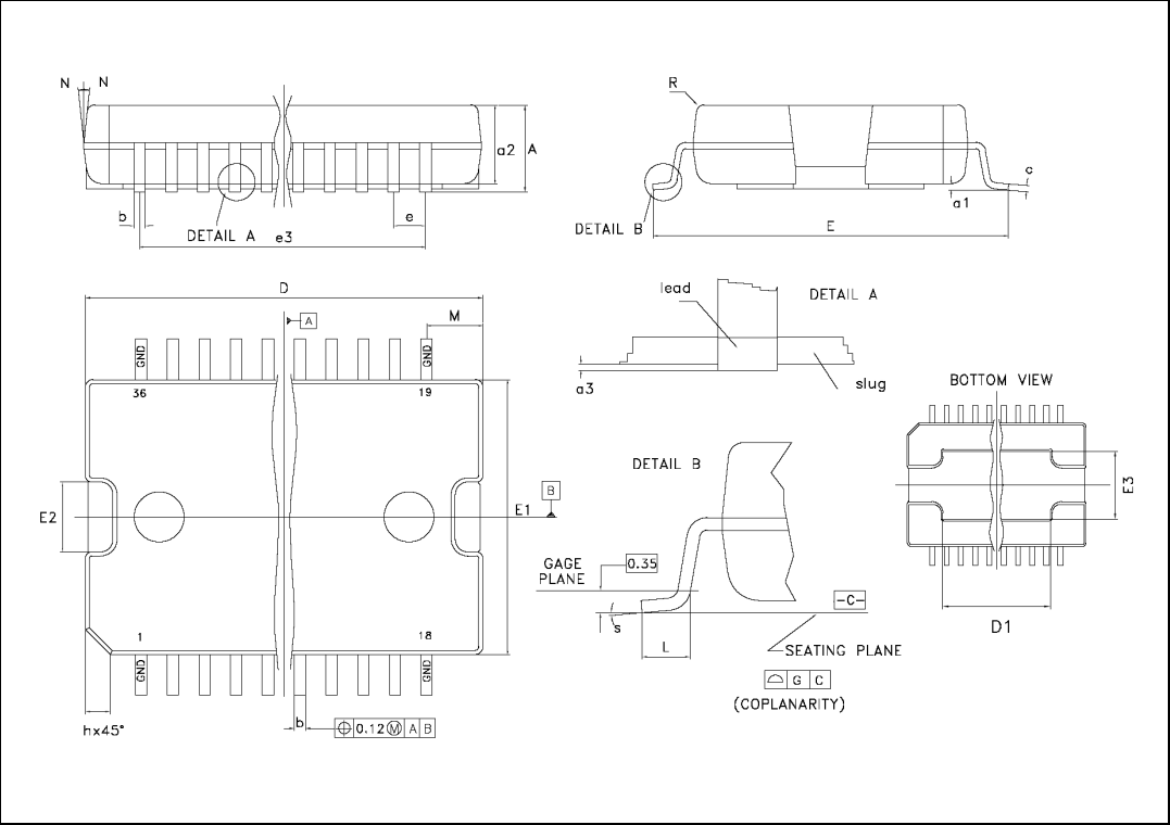
Figure 9. PowerSO-36 drawings
