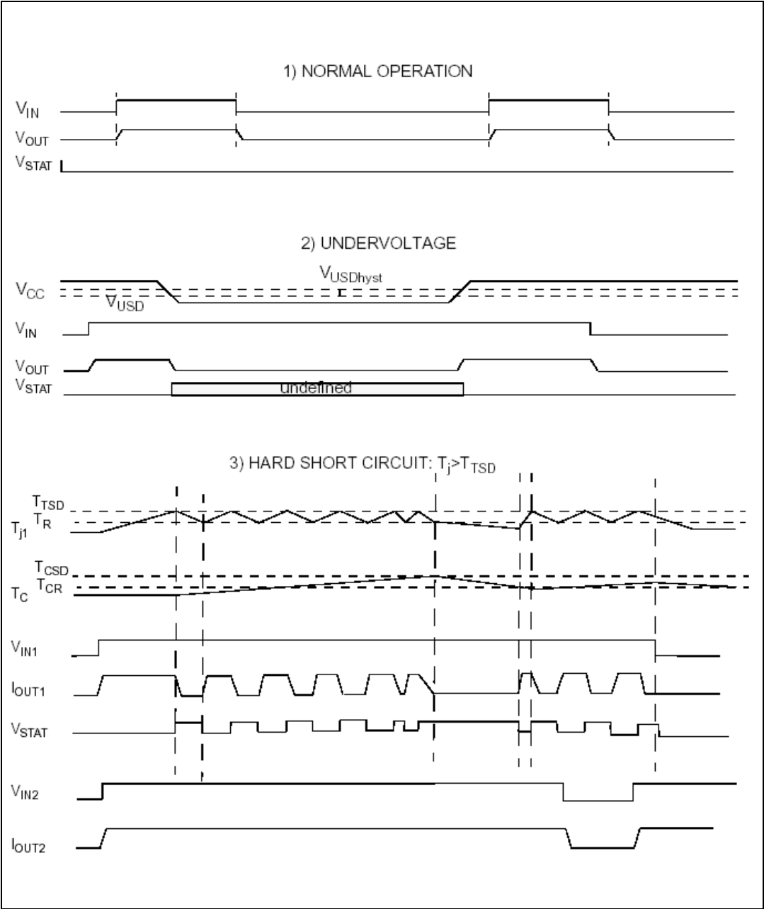
Figure 7. Waveforms
