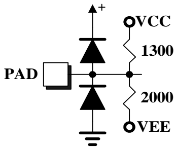
VCOM (L or R) Input Equivalent Circuit
