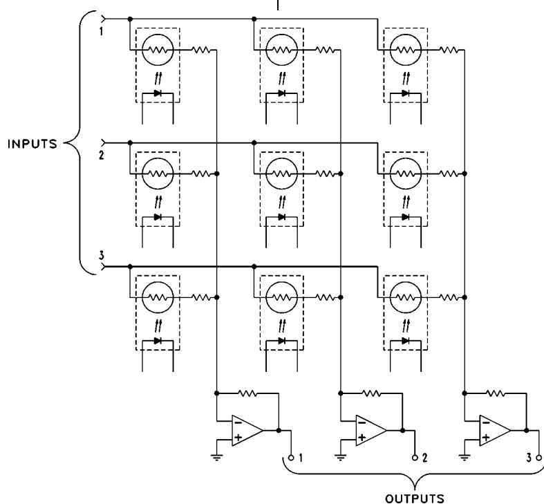
Figure 2. Switching Matrix
