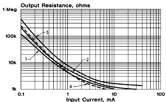
Output Resistance vs. Input Current VTL5C8
