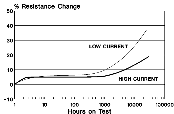
Figure 5. VTL5C3 Life Test.
