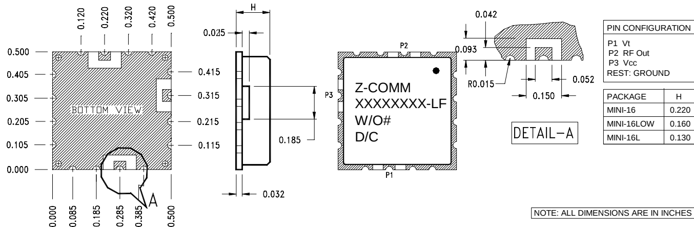
PHYSICAL DIMENSIONS
