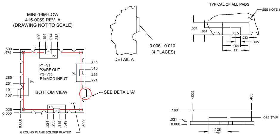
PHYSICAL DIMENSIONS
