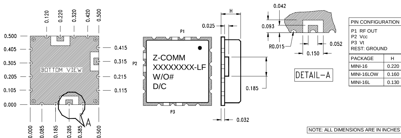
PHYSICAL DIMENSIONS
